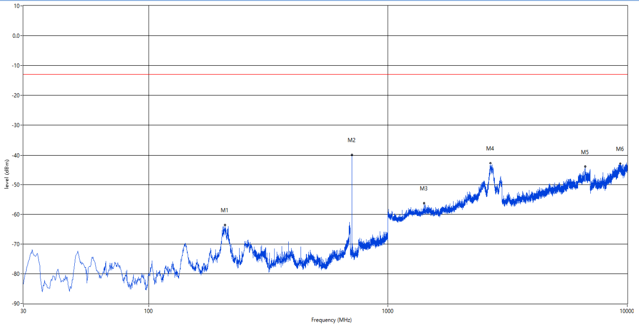
RSE-H 1.4wid 30MHz-10GHz MID
