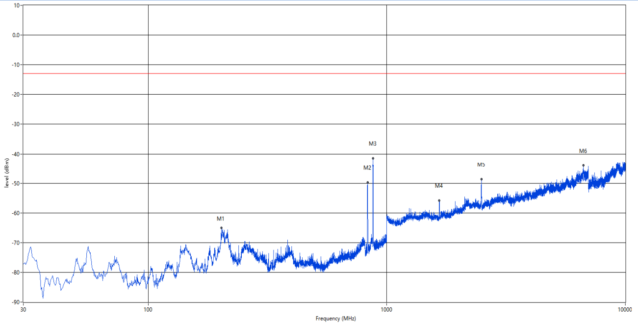
RSE-H 5wid 30MHz-10GHz MID
