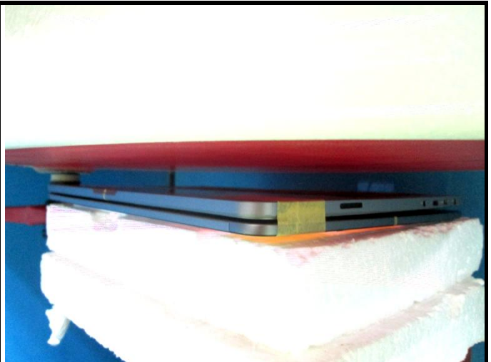
Body - Rear Face of EUT at 20 mm
