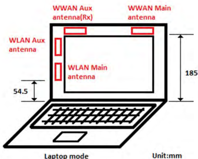
Fig.7 Antenna position of EUT(laptop mode)
