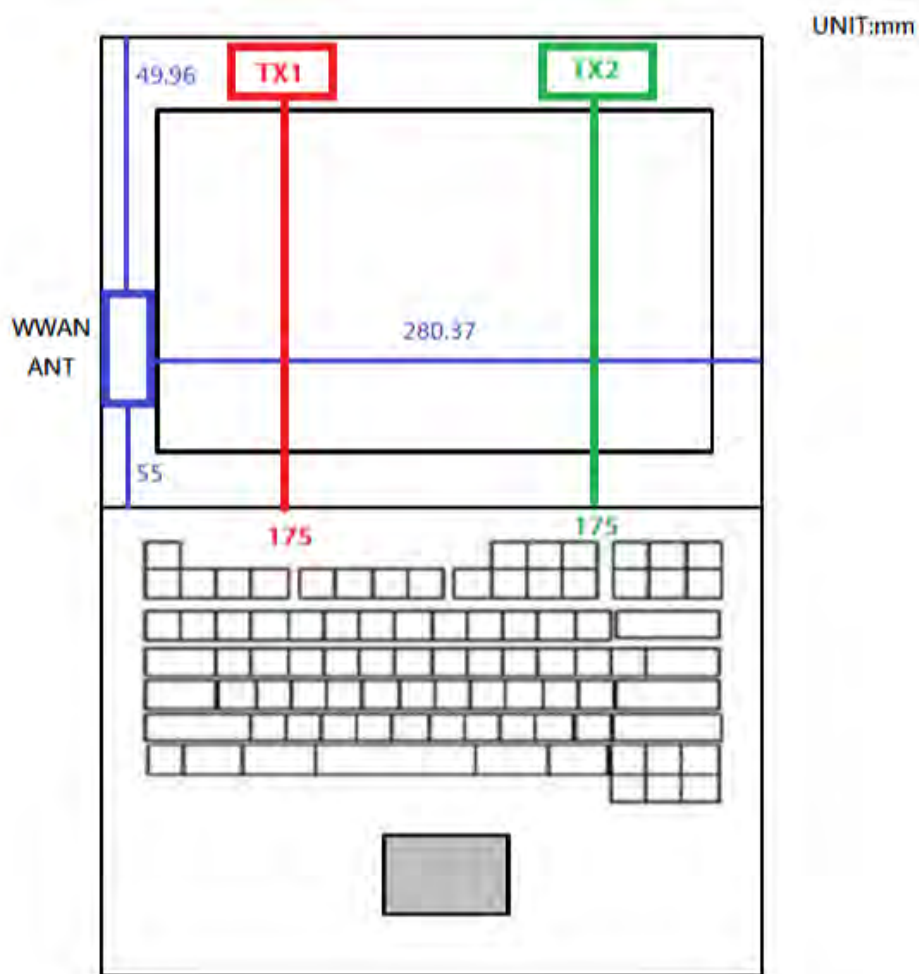
Fig.6 Antenna location
