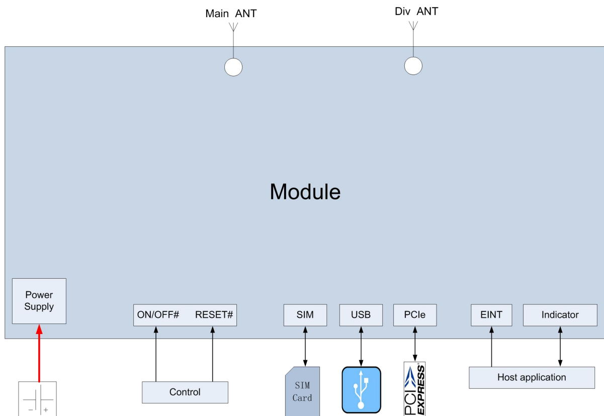
Figure2-1 Application Framework
