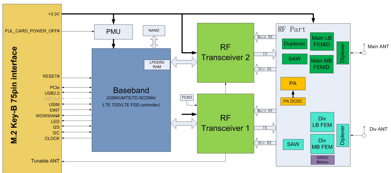
Figure 2-2 Hardware Framework
