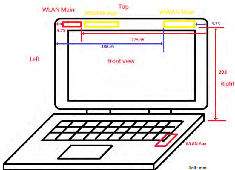
Fig.12 Antenna location (Notebook mode)
