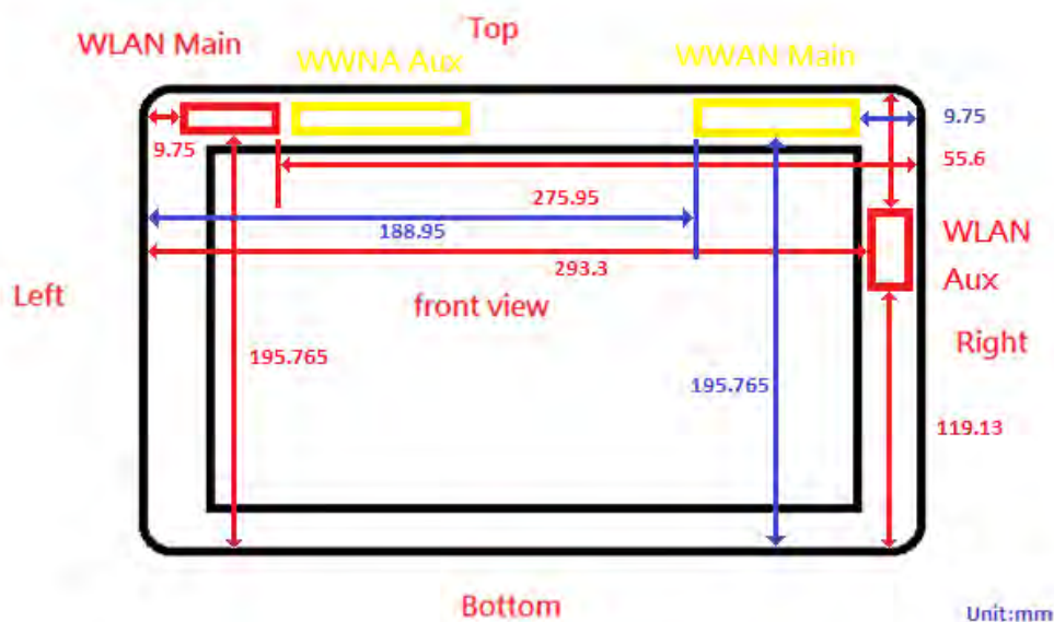
Fig.11 Antenna location (Tablet mode)
