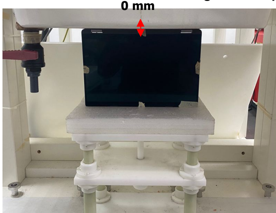
Fig.5 EUT Bottom side (Tablet mode) to flat phantom
