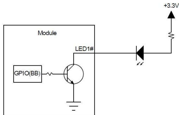
Figure 3-14 LEDDriving Circuit
