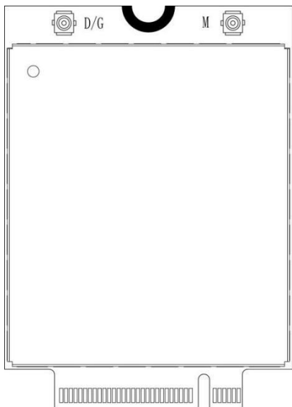
Figure 4-1 RF connectors
