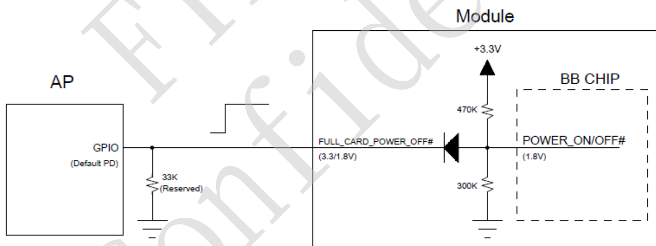
Figure 3-4 Circuit for module start-up controlled by AP
