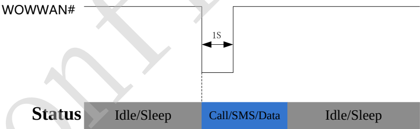
Figure 3-18 WOWWAN# timing
