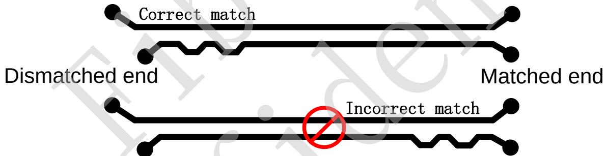
Figure 3-14 Length match design of PCIe differential pair
