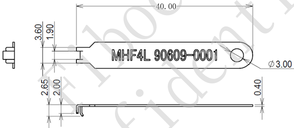
Figure 4-6 Pulling JIG
