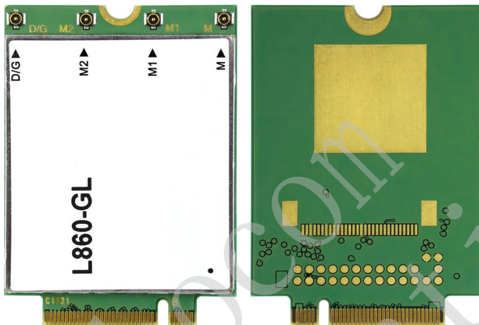
Figure 6-1 Module appearance
