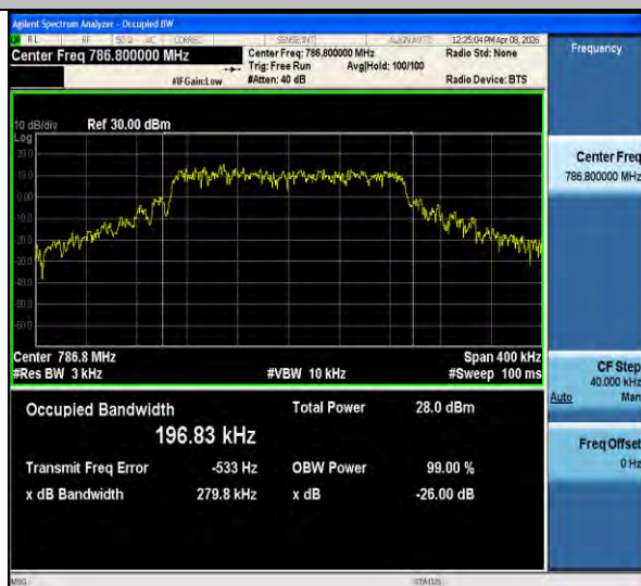
Band13-0.18-QPSK-23278-PASS
