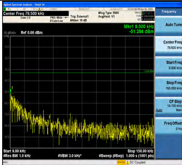
Band13-0.18-BPSK-23182-30-1000-PASS
