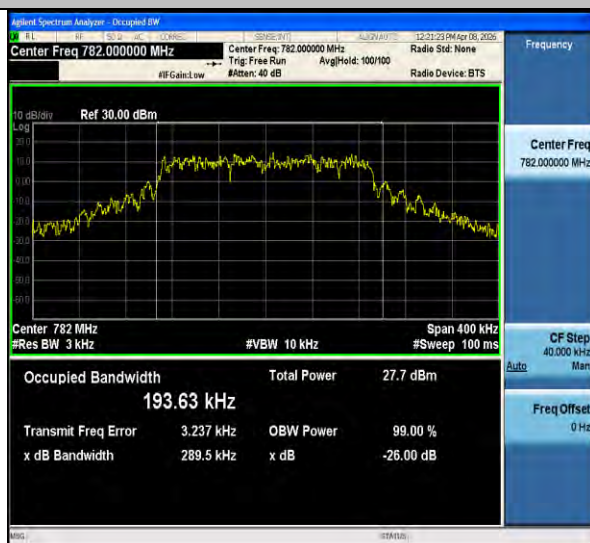
Band13-0.18-QPSK-23230-PASS
