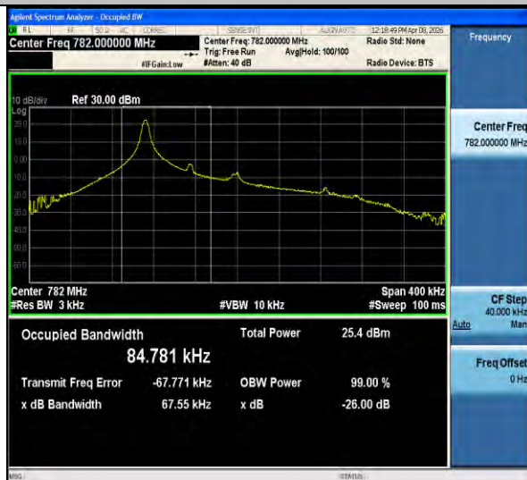
Band13-0.18-QPSK-23230-PASS
