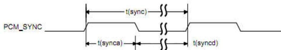
Figure 3-17 PCM_SYNC Timing
