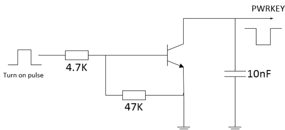
Figure 3-4 OC/OD Drive Power on Reference Circuit
