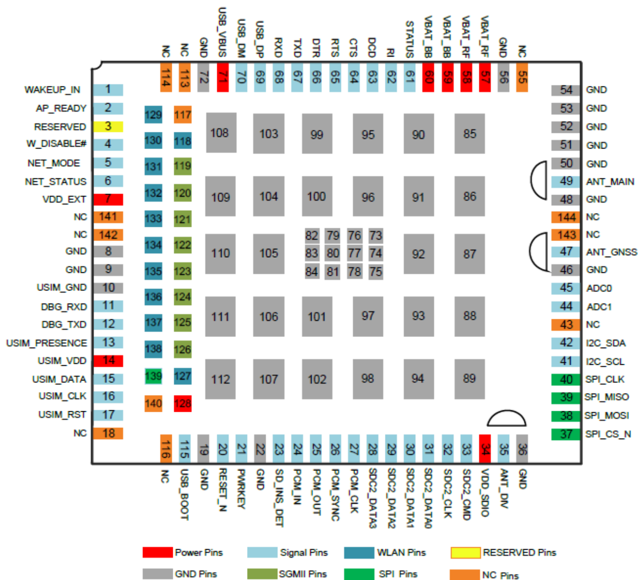
Figure 3-1 Pin Distribution Diagram(TOP plan perspective diagram)
