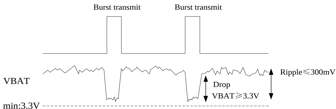
Figure 3-3 Power Limit
