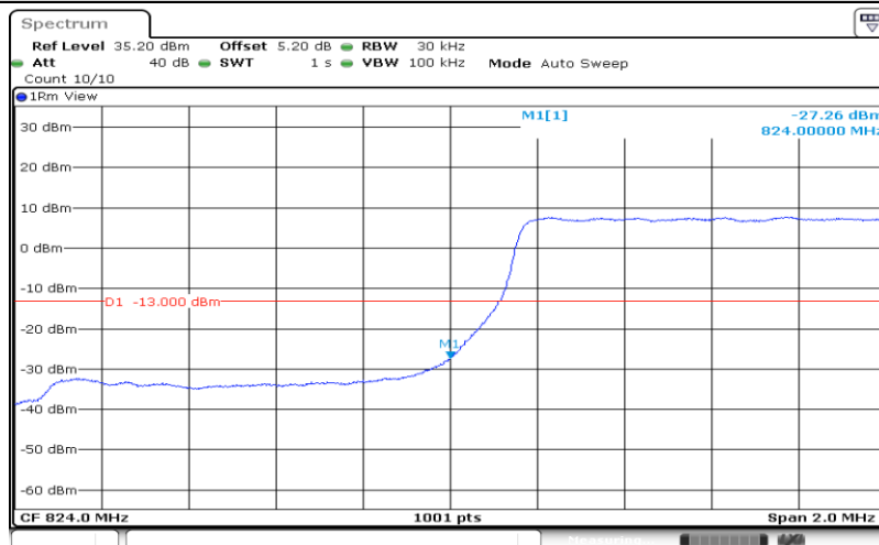
Band5-1.4MHz-QPSK-20407-6RB#0
