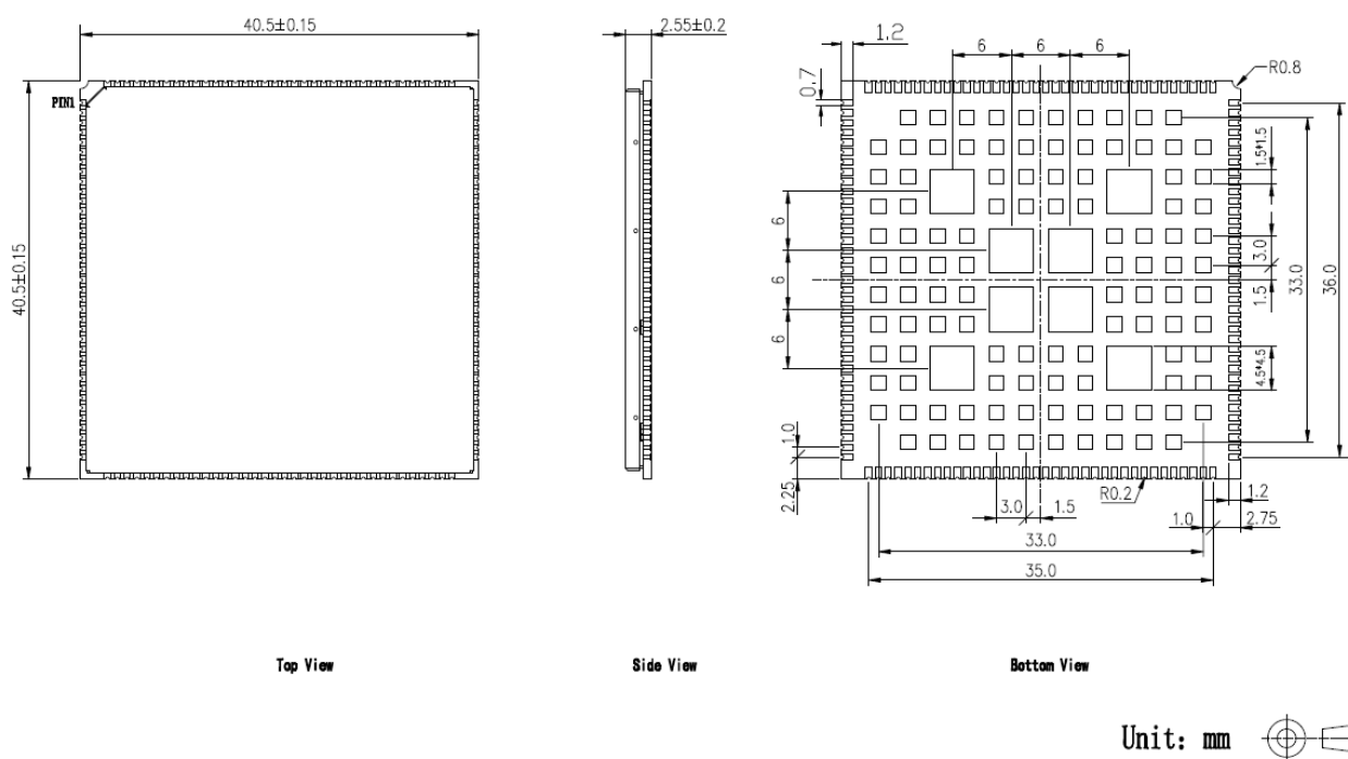
Figure 34. Structural dimensions
