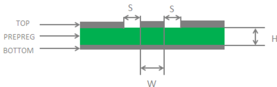
Figure 30. Two-layer PCB coplanar waveguide structure
