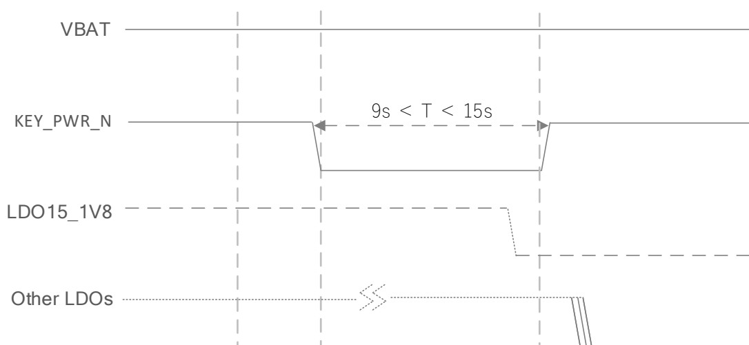
Figure 10. Power-off timing
