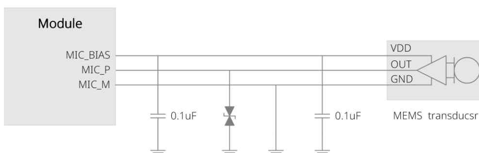
Figure 21. Microphone circuit design
