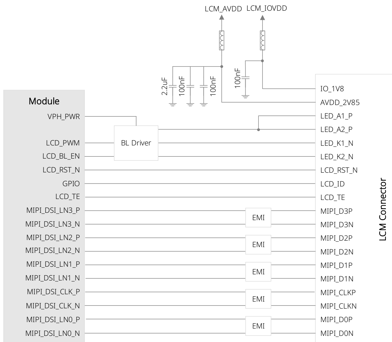
Figure 16. LCD reference circuit
