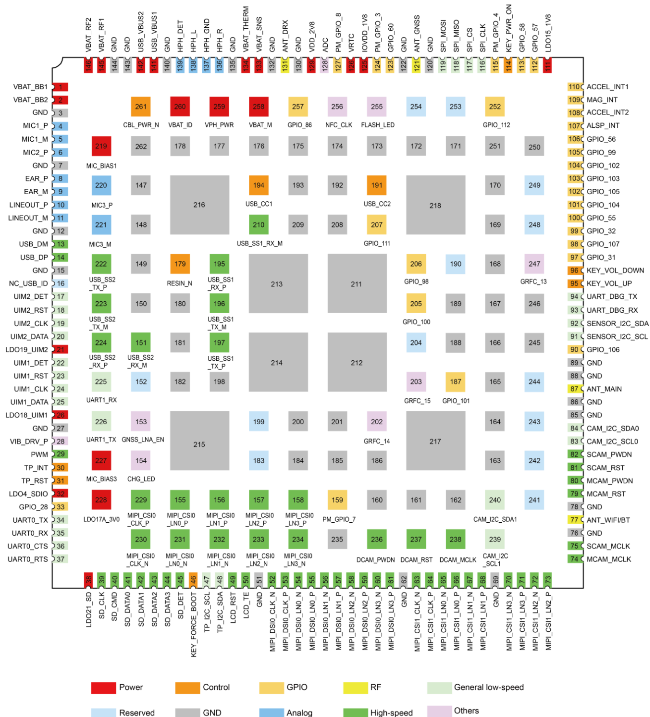
Figure 2. Pin distribution
