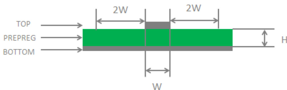
Figure 29. Two-layer PCB microstrip line structure
