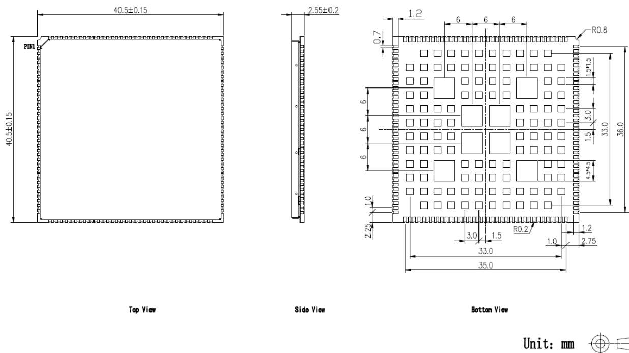
Figure 29. Structure dimensions
