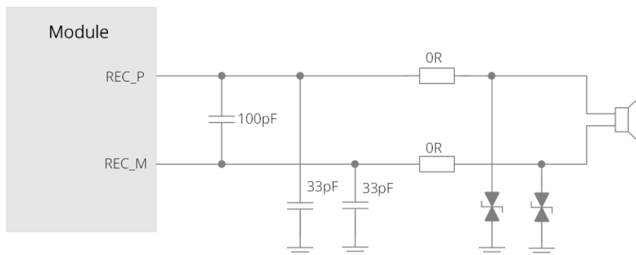
Figure 20. Receiver circuit design
