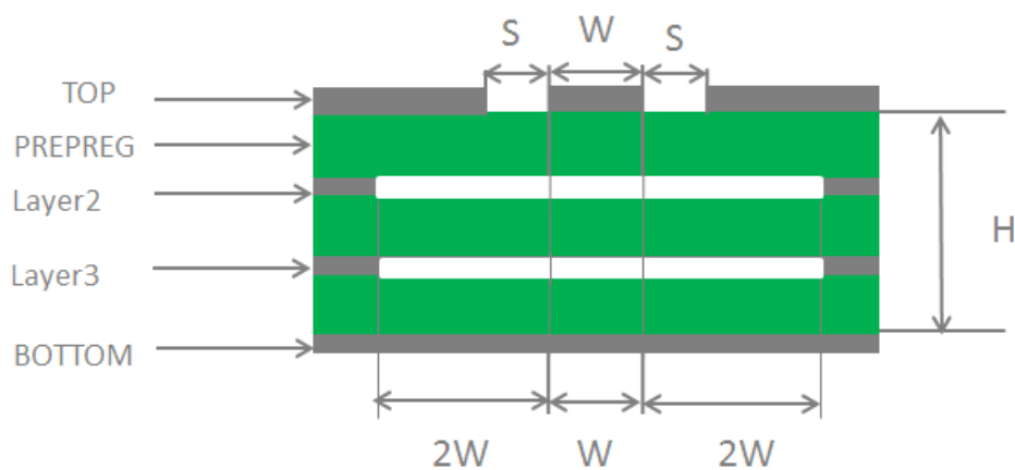
Figure 27. Four-layer PCB coplanar waveguide structure (see ground layer 4)
