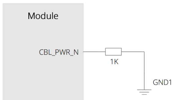
Figure 8. CBL power-on reference circuit
