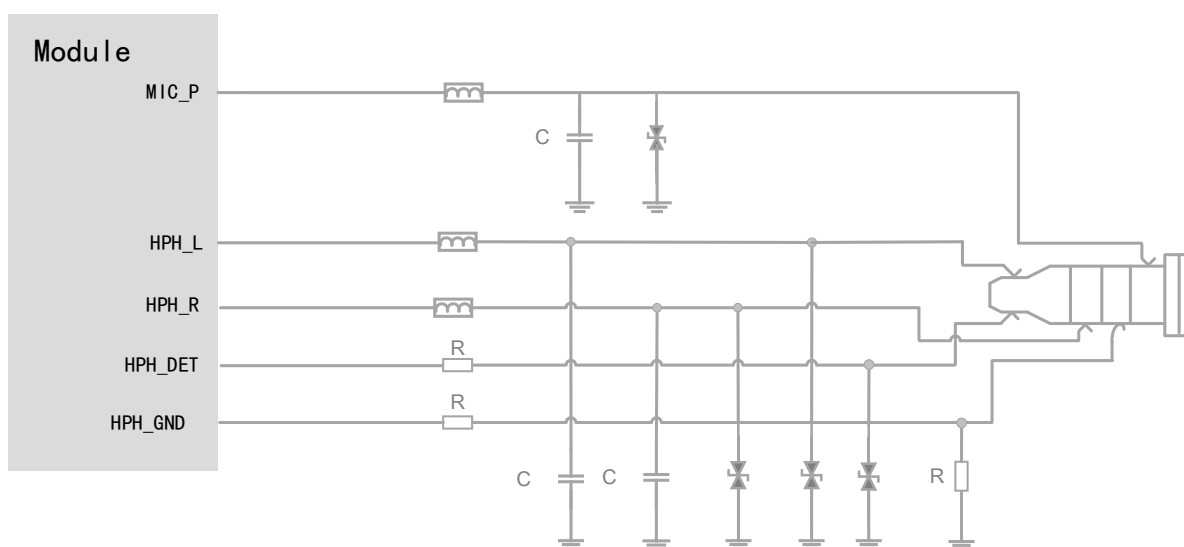
Figure 21. Headphone interface circuit design
