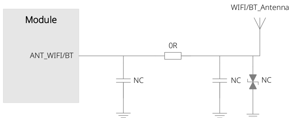
Figure 23. Antenna reference circuit
