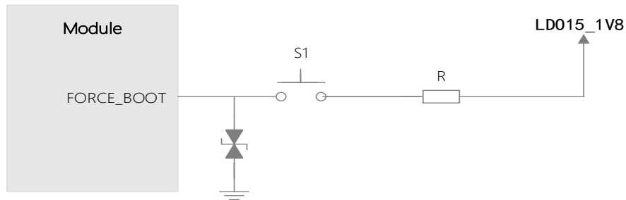
Figure 22. Design of forced download interface
