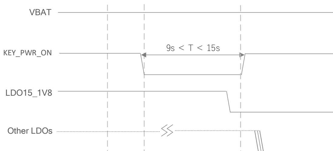
Figure 10. Power-off timing
