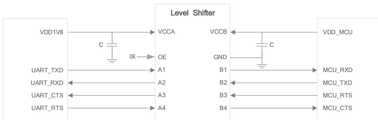
Figure 12. Level conversion reference circuit
