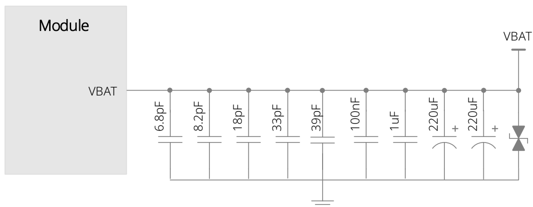
Figure 4. Reference design of power circuit
