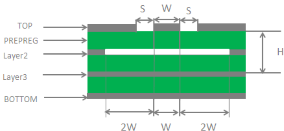
Figure 26 Four-layer PCB coplanar waveguide structure (see ground layer 3)
