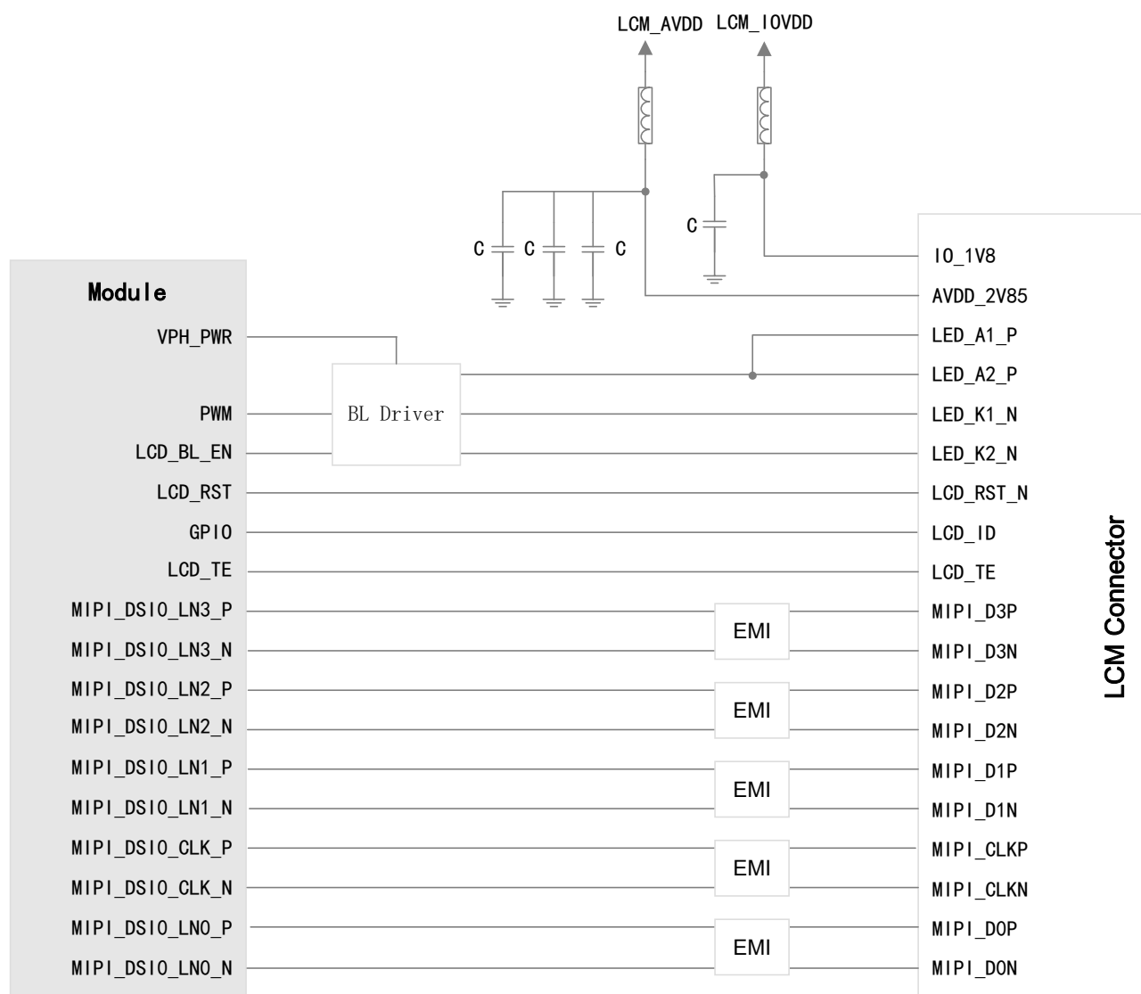
Figure 14. LCD reference circuit
