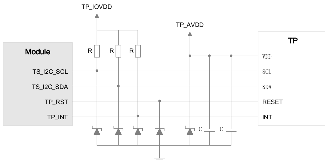
Figure 15. TP reference circuit design
