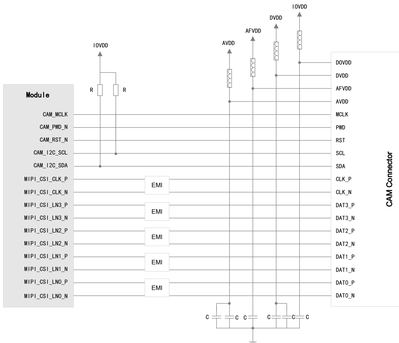
Figure 16. Reference circuit design of camera 0
