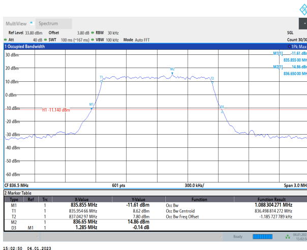
Band26-1.4MHz-QPSK-26915-6RB#0
