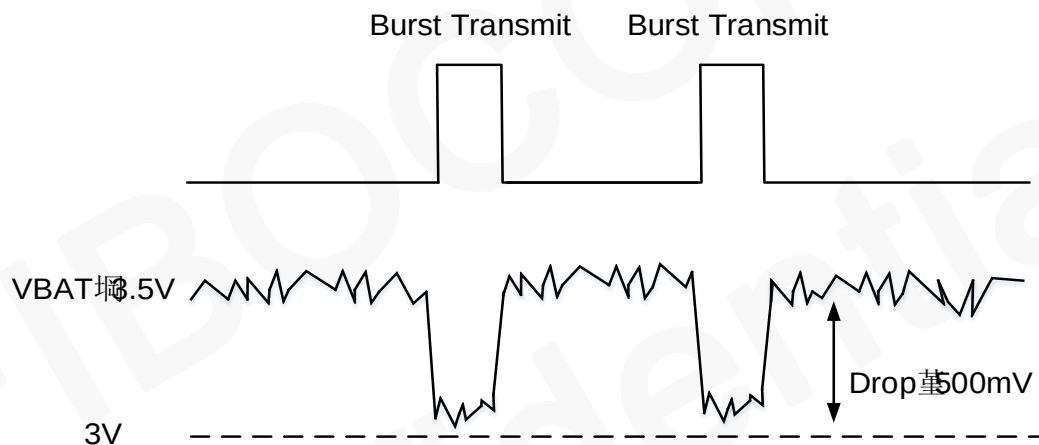
Figure 3-1 Voltage drop
