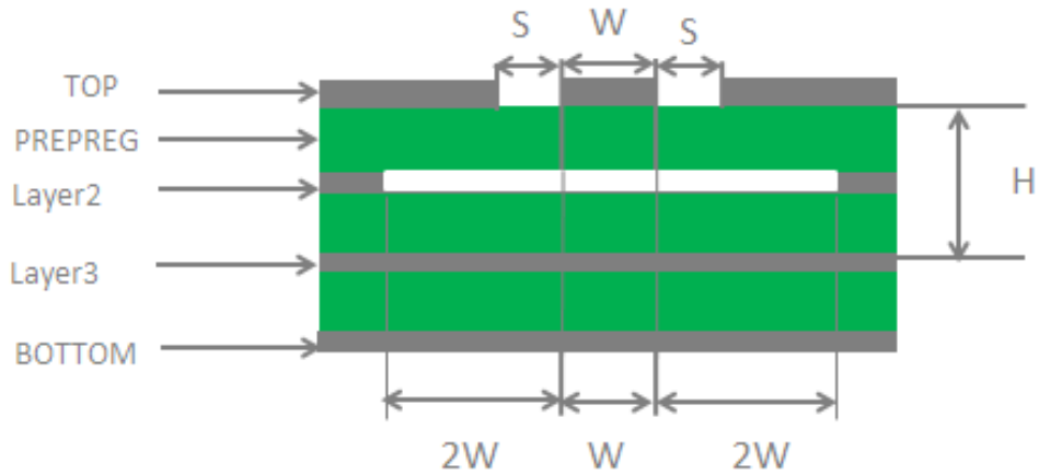
Figure 4-3 Coplanar waveguide structure of four-layer PCB (reference ground layer 3)
