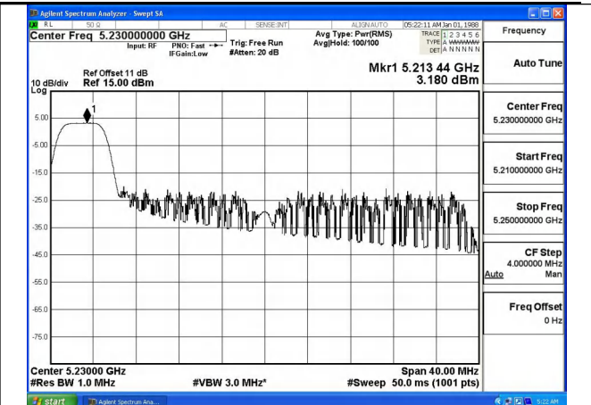
Mode:802.11ax HE40 Tone:52T Frequency:5230MHz Ant:Chain1
