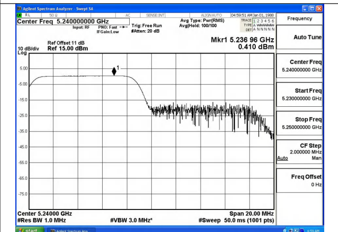
Mode:802.11ax HE20 Tone:106T Frequency:5240MHz Ant:Chain1
