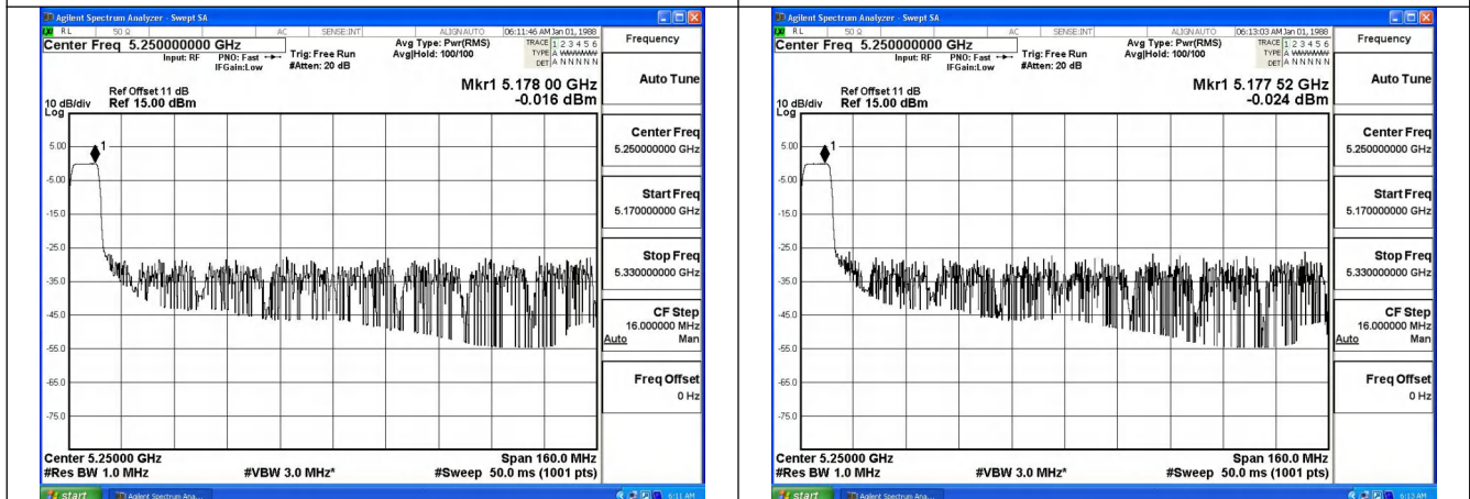
Mode:802.11ax HE160 Tone:106T Frequency:5250MHz Ant:Chain0
