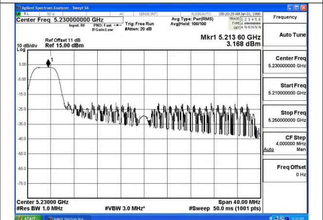
Mode:802.11ax HE40 Tone:52T Frequency:5230MHz Ant:Chain0
