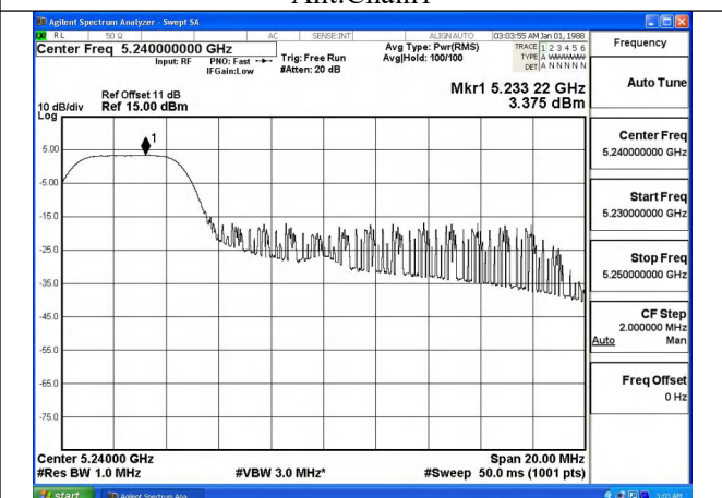
Mode:802.11ax HE20 Tone:52T Frequency:5240MHz Ant:Chain1
