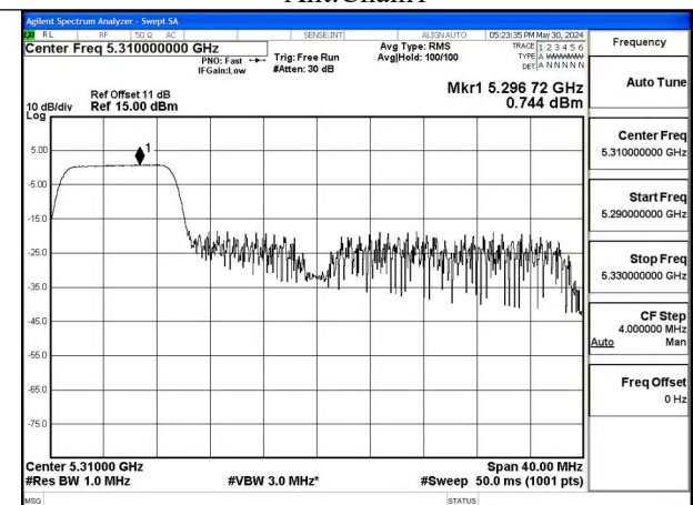
Mode:802.11ax HE40 Tone:106T Frequency:5310MHz Ant:Chain0
