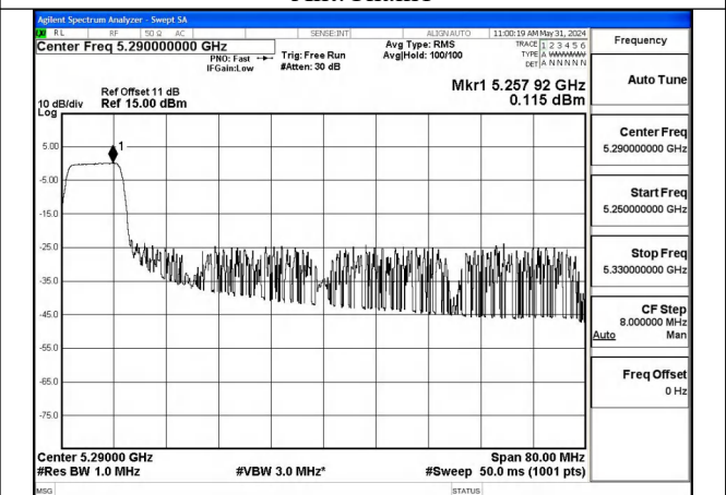
Mode:802.11ax HE80 Tone:106T Frequency:5290MHz Ant:Chain1
