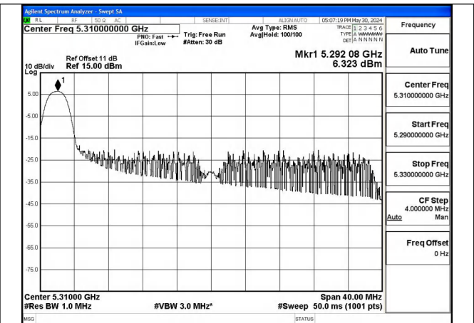
Mode:802.11ax HE40 Tone:26T Frequency:5310MHz Ant:Chain0
