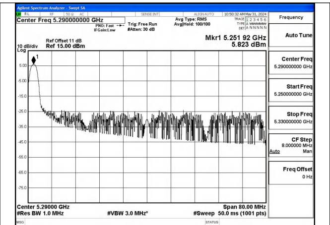
Mode:802.11ax HE80 Tone:26T Frequency:5290MHz Ant:Chain1
