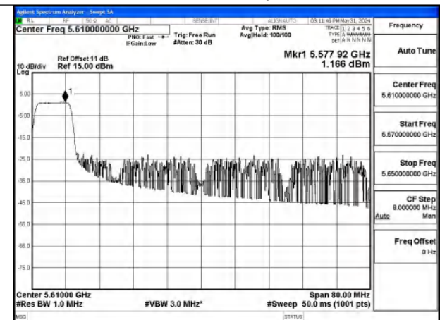
Mode:802.11ax HE80 Tone:106T Frequency:5610MHz Ant:Chain1
