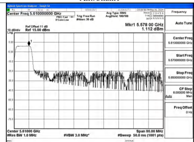
Mode:802.11ax HE80 Tone:106T Frequency:5610MHz Ant:Chain0
