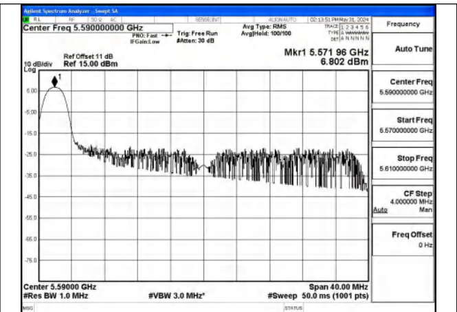
Mode:802.11ax HE40 Tone:26T Frequency:5590MHz Ant:Chain0
