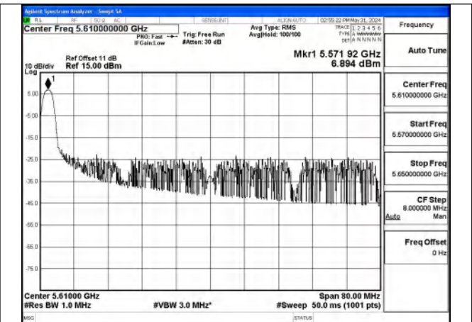
Mode:802.11ax HE80 Tone:26T Frequency:5610MHz Ant:Chain0
