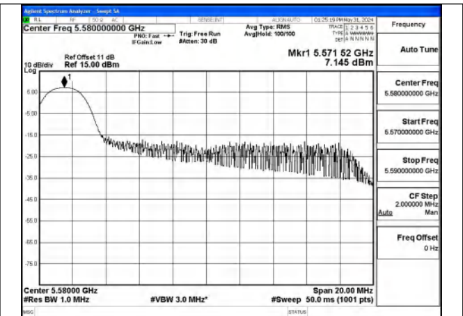
Mode:802.11ax HE20 Tone:26T Frequency:5580MHz Ant:Chain0
