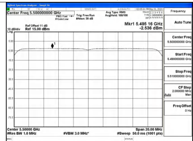
Mode:802.11ax HE20 Tone:242T Frequency:5500MHz Ant:Chain1
