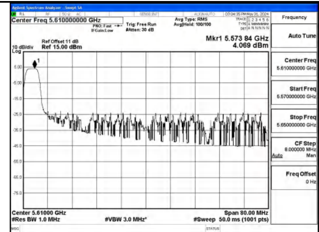
Mode:802.11ax HE80 Tone:52T Frequency:5610MHz Ant:Chain1
