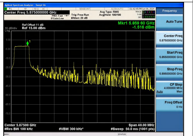
Mode:802.11ax HE40 Tone:52T Frequency:5875MHz Ant:Chain1
