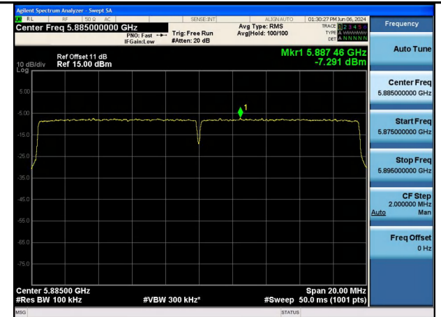
Mode:802.11ax HE20 Tone:242T Frequency:5885MHz Ant:Chain0
