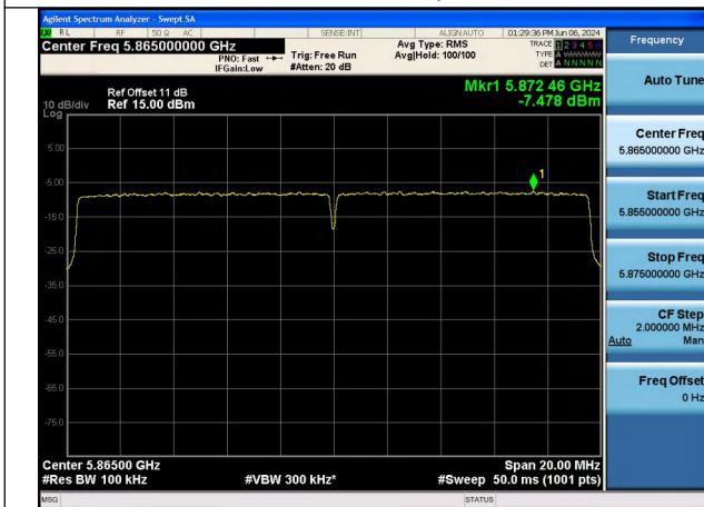
Mode:802.11ax HE20 Tone:242T Frequency:5865MHz Ant:Chain1
