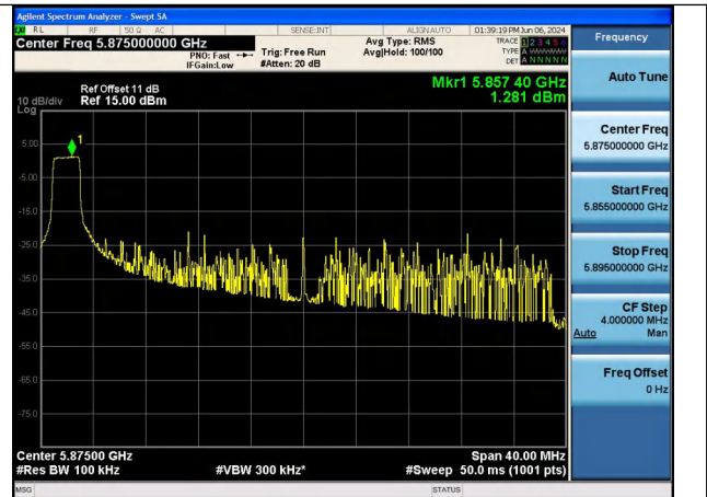
Mode:802.11ax HE40 Tone:26T Frequency:5875MHz Ant:Chain1
