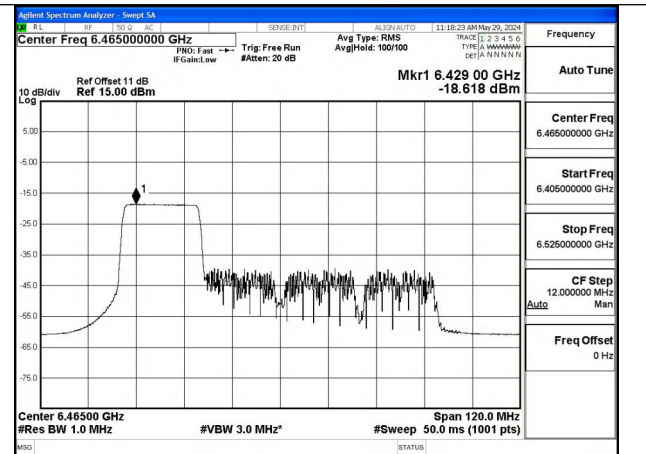
Mode:802.11ax HE80 Tone:242T Frequency:6465MHz Ant:Chain1
