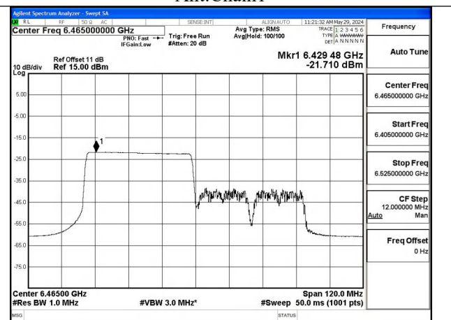
Mode:802.11ax HE80 Tone:484T Frequency:6465MHz Ant:Chain1
