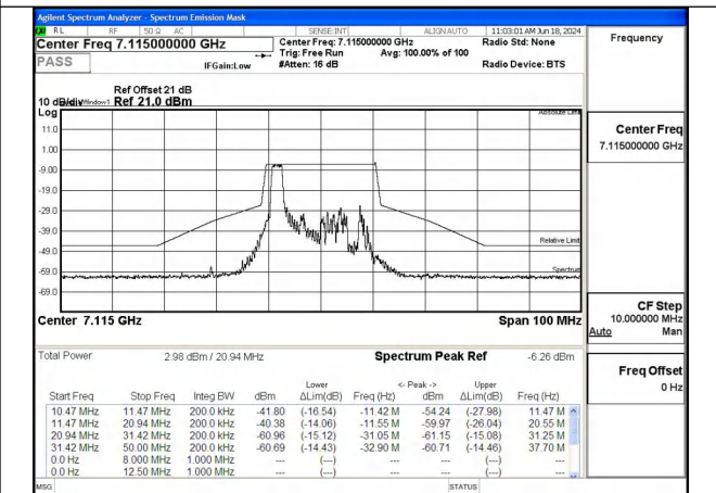
Mode:802.11ax HE20 Tone:26T Frequency:7115MHz Ant:Chain1
