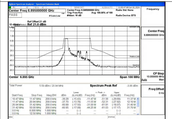
Mode:802.11ax HE20 Tone:26T Frequency:6895MHz Ant:Chain1
