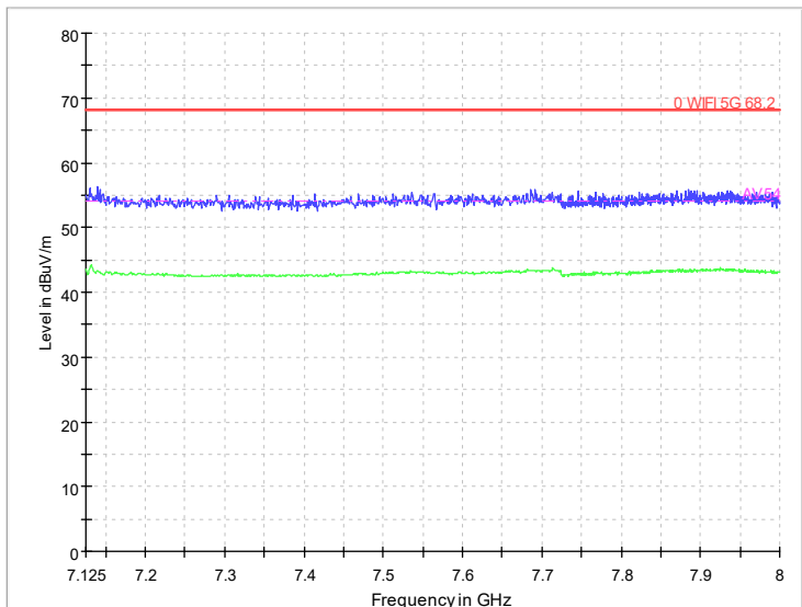
Radiated Emission Band Edge Channel No.:215 Test Mode: 802.11ax(HE80) Polarization: V
