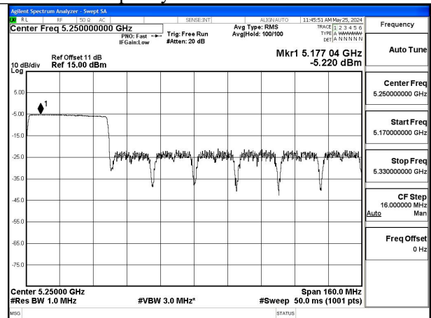
Mode:802.11ax HE160 Tone:484T Frequency:5250MHz Ant:Chain1
