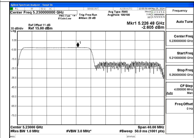
Mode:802.11ax HE40 Tone:242T Frequency:5230MHz Ant:Chain1
