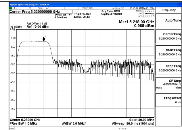
Mode:802.11ax HE40 Tone:106T Frequency:5230MHz Ant:Chain0
