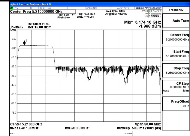
Mode:802.11ax HE80 Tone:242T Frequency:5210MHz Ant:Chain1
