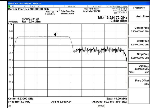
Mode:802.11ax HE40 Tone:242T Frequency:5230MHz Ant:Chain0
