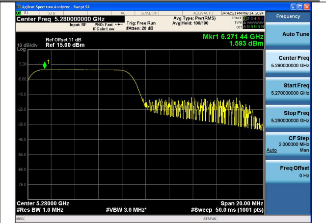
Mode:802.11ax HE20 Tone:106T Frequency:5280MHz Ant:Chain0
