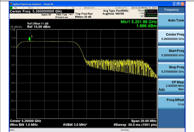
Mode:802.11ax HE20 Tone:106T Frequency:5260MHz Ant:Chain1
