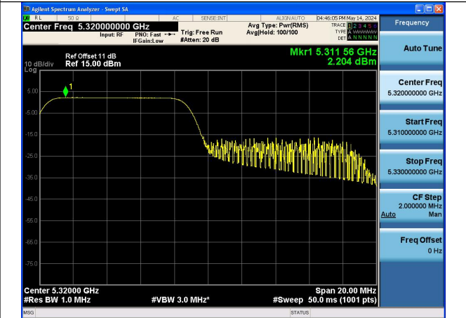
Mode:802.11ax HE20 Tone:106T Frequency:5320MHz Ant:Chain1
