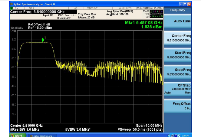
Mode:802.11ax HE40 Tone:106T Frequency:5510MHz Ant:Chain1
