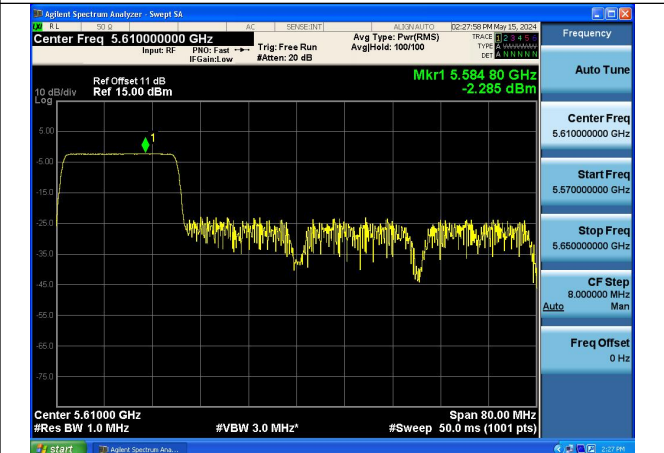
Mode:802.11ax HE80 Tone:242T Frequency:5610MHz Ant:Chain1
