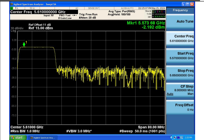
Mode:802.11ax HE80 Tone:242T Frequency:5610MHz Ant:Chain0
