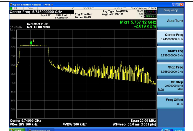
Mode:802.11ax HE20 Tone:52T Frequency:5745MHz Ant:Chain1
