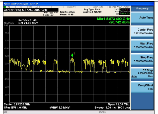
Mode:802.11ax HE80 Tone:26TR Frequency:5855MHz Ant:Chain1 scope:NII4
