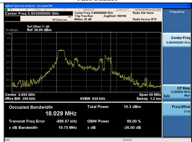
Mode:802.11ax HE20 TONE:26T Frequency:5955MHz Ant:Chain1
