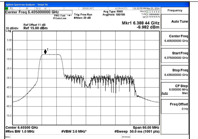
Mode:802.11ax HE40 Tone:106T Frequency:6405MHz Ant:Chain1
