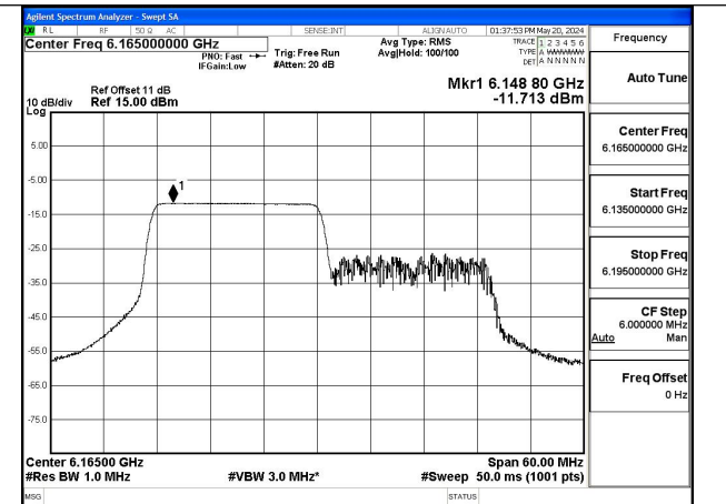
Mode:802.11ax HE40 Tone:242T Frequency:6165MHz Ant:Chain0
