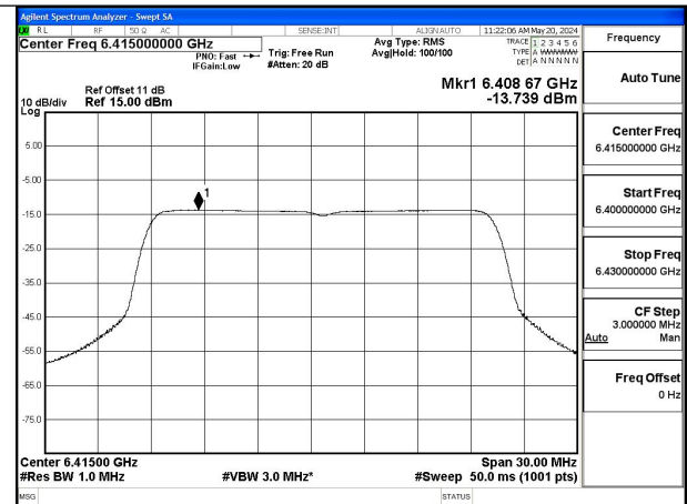
Mode:802.11ax HE20 Tone:242T Frequency:6415MHz Ant:Chain1
