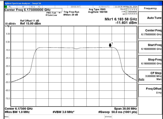
Mode:802.11ax HE20 Tone:242T Frequency:6175MHz Ant:Chain0
