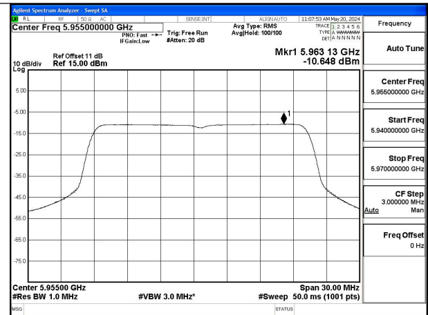
Mode:802.11ax HE20 Tone:242T Frequency:5955MHz Ant:Chain1
