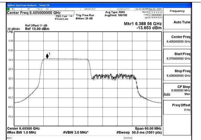
Mode:802.11ax HE40 Tone:242T Frequency:6405MHz Ant:Chain1
