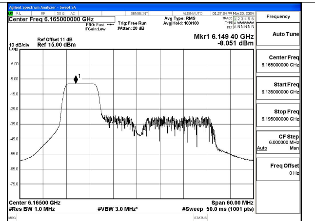
Mode:802.11ax HE40 Tone:106T Frequency:6165MHz Ant:Chain0
