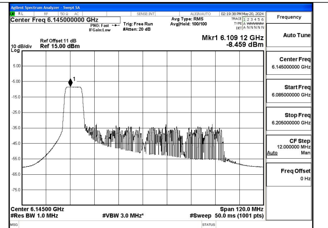
Mode:802.11ax HE80 Tone:106T Frequency:6145MHz Ant:Chain0
