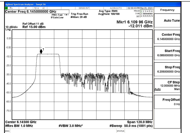
Mode:802.11ax HE80 Tone:242T Frequency:6145MHz Ant:Chain0
