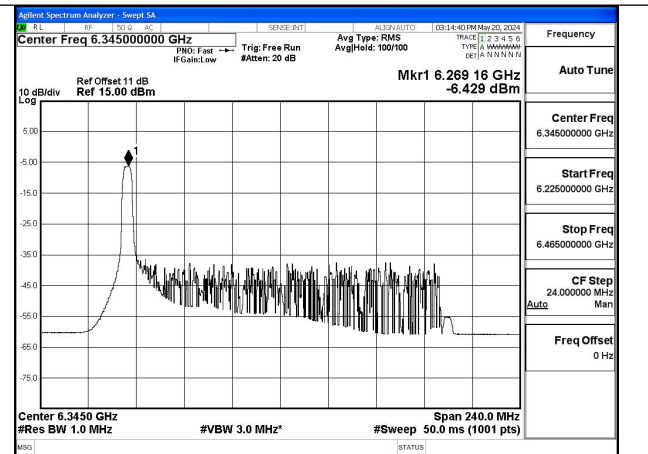
Mode:802.11ax HE160 Tone:52T Frequency:6345MHz Ant:Chain1
