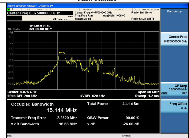
Mode:802.11ax HE20 TONE:26T Frequency:6875MHz Ant:Chain1
