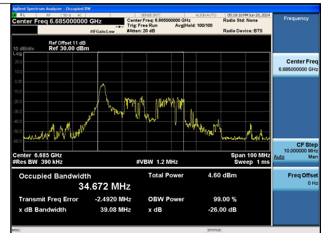
Mode:802.11ax HE40 TONE:26T Frequency:6685MHz Ant:Chain0
