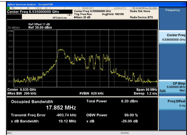
Mode:802.11ax HE20 TONE:26T Frequency:6535MHz Ant:Chain1
