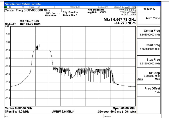
Mode:802.11ax HE40 Tone:106T Frequency:6685MHz Ant:Chain0
