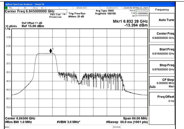
Mode:802.11ax HE40 Tone:106T Frequency:6845MHz Ant:Chain1
