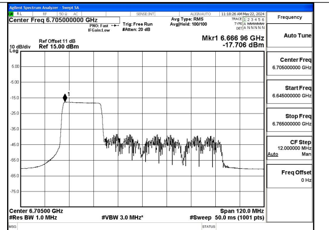
Mode:802.11ax HE80 Tone:242T Frequency:6705MHz Ant:Chain0
