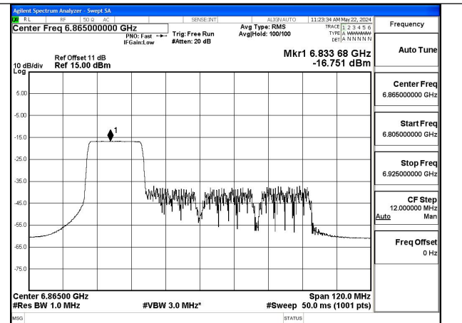
Mode:802.11ax HE80 Tone:242T Frequency:6865MHz Ant:Chain1
