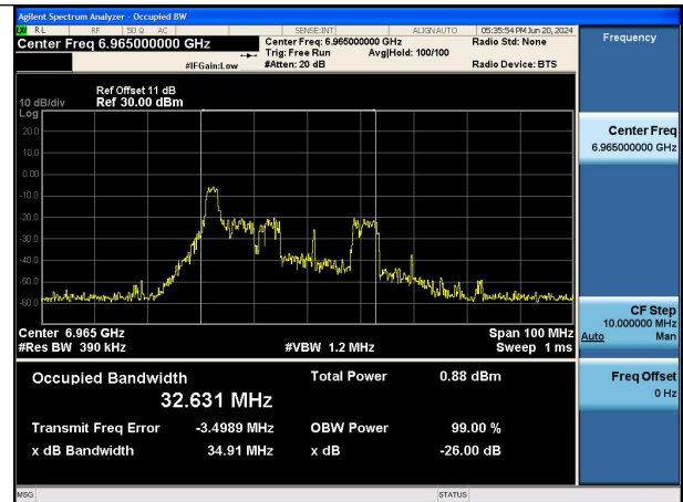
Mode:802.11ax HE40 TONE:26T Frequency:6965MHz Ant:Chain0
