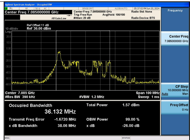
Mode:802.11ax HE40 TONE:26T Frequency:7085MHz Ant:Chain1
