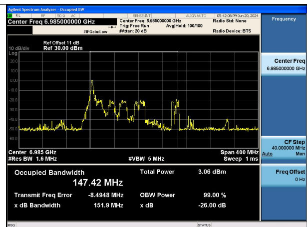
Mode:802.11ax HE160 TONE:26T Frequency:6985MHz Ant:Chain1
