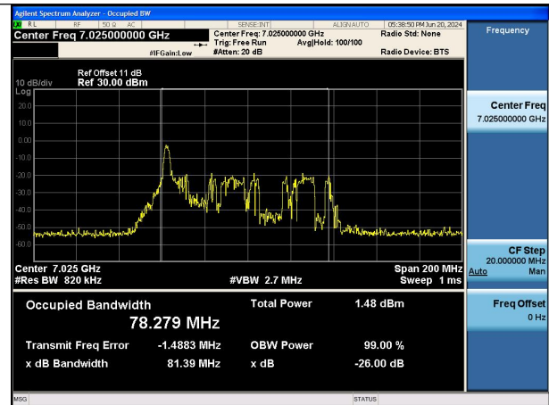
Mode:802.11ax HE80 TONE:26T Frequency:7025MHz Ant:Chain0
