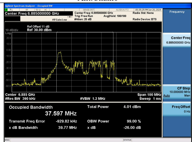
Mode:802.11ax HE40 TONE:26T Frequency:6885MHz Ant:Chain1
