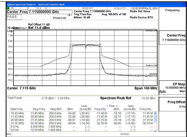
Mode:802.11ax HE20 Tone:242T Frequency:7115MHz Ant:Chain1
