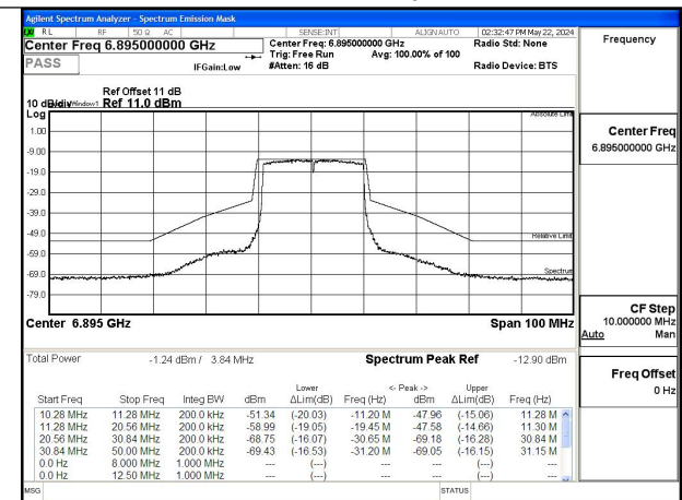
Mode:802.11ax HE20 Tone:242T Frequency:6895MHz Ant:Chain1
