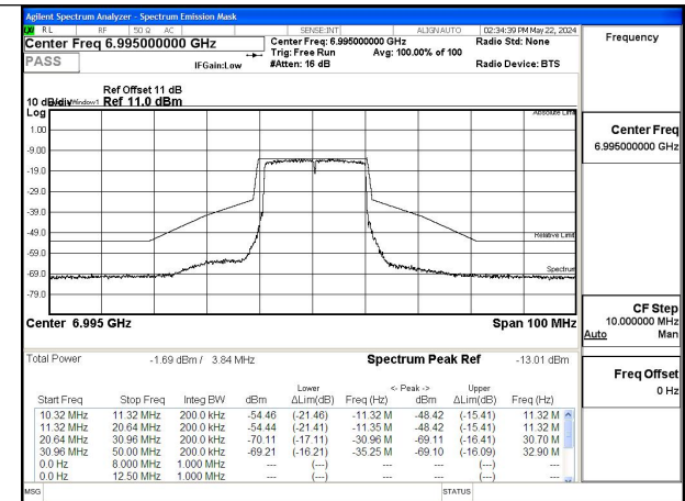
Mode:802.11ax HE20 Tone:242T Frequency:6995MHz Ant:Chain0
