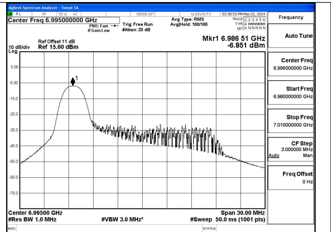
Mode:802.11ax HE20 Tone:26T Frequency:6995MHz Ant:Chain0
