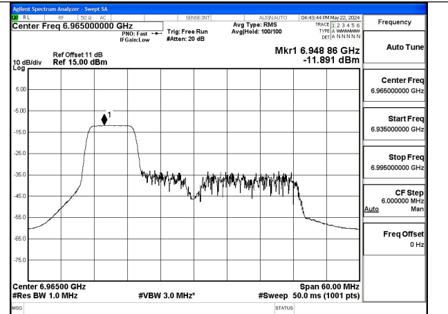
Mode:802.11ax HE40 Tone:106T Frequency:6965MHz Ant:Chain0
