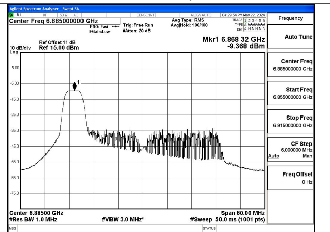
Mode:802.11ax HE40 Tone:52T Frequency:6885MHz Ant:Chain1
