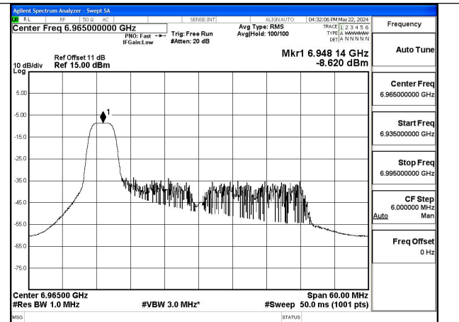
Mode:802.11ax HE40 Tone:52T Frequency:6965MHz Ant:Chain0
