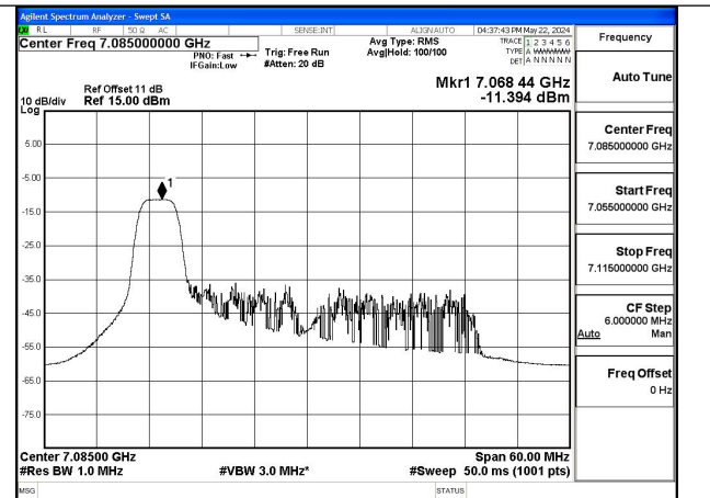
Mode:802.11ax HE40 Tone:52T Frequency:7085MHz Ant:Chain1
