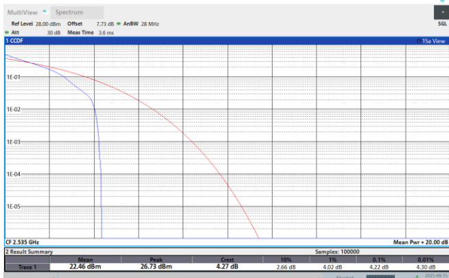
Band7-20MHz-QPSK-21350-1RB#0
