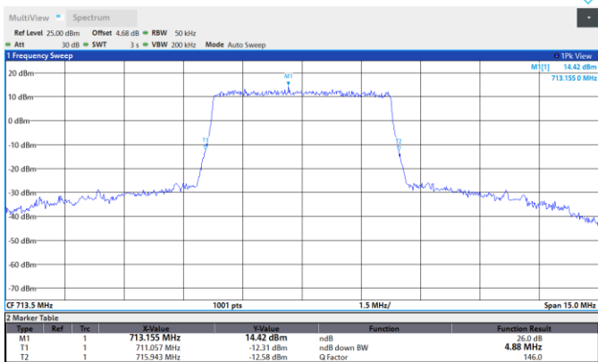
Band12-5MHz-16QAM-23095-25RB#0
