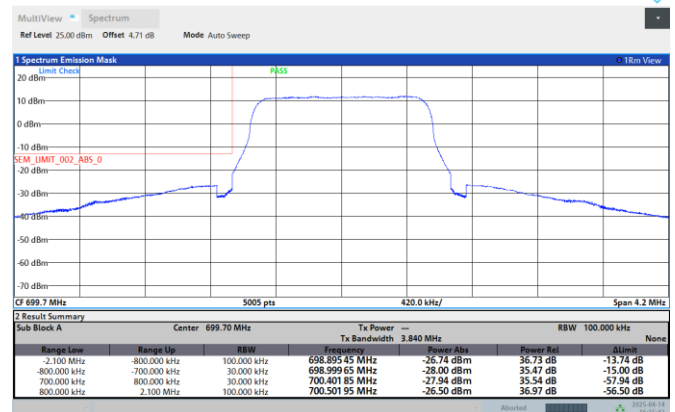
Band12-1.4MHz-16QAM-23173-6RB#0
