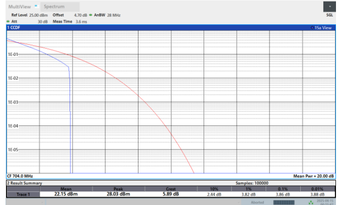
Band12-10MHz-QPSK-23095-50RB#0
