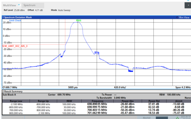
Band12-1.4MHz-16QAM-23173-1RB#5
