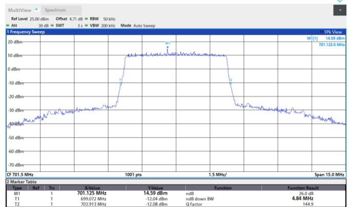
Band12-5MHz-16QAM-23155-25RB#0
