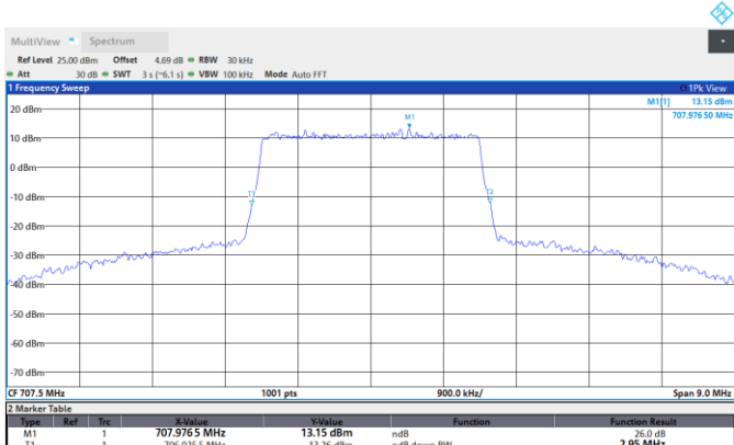
Band12-3MHz-16QAM-23095-15RB#0
