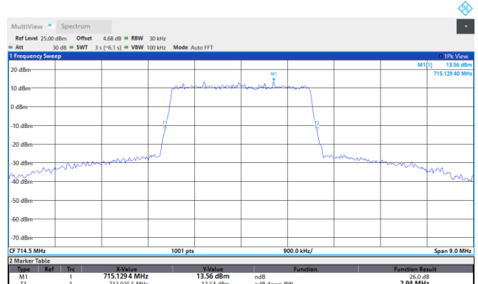
Band12-3MHz-16QAM-23165-15RB#0
