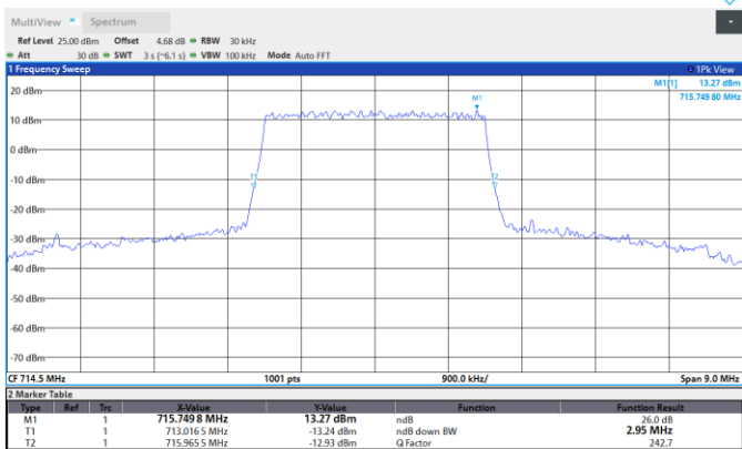
Band12-3MHz-16QAM-23095-15RB#0
