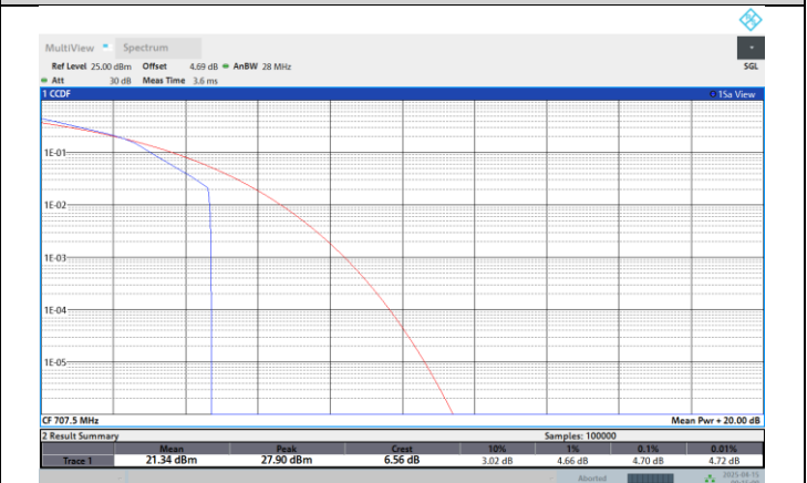
Band12-5MHz-16QAM-23155-25RB#0
