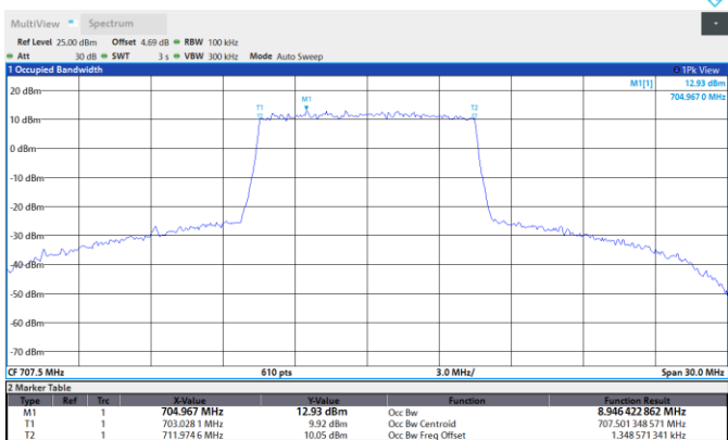
Band12-10MHz-16QAM-23095-50RB#0
