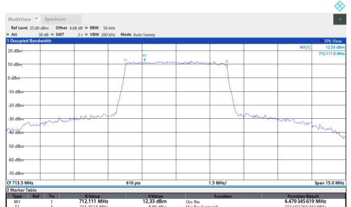
Band12-5MHz-16QAM-23155-25RB#0
