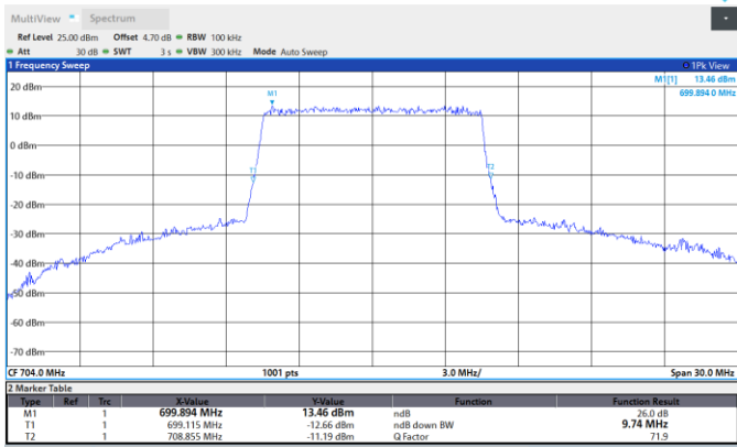
Band12-10MHz-QPSK-23095-50RB#0
