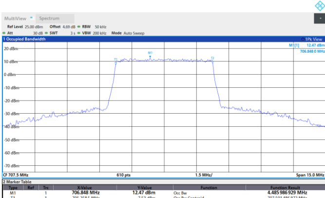
Band12-5MHz-16QAM-23095-25RB#0
