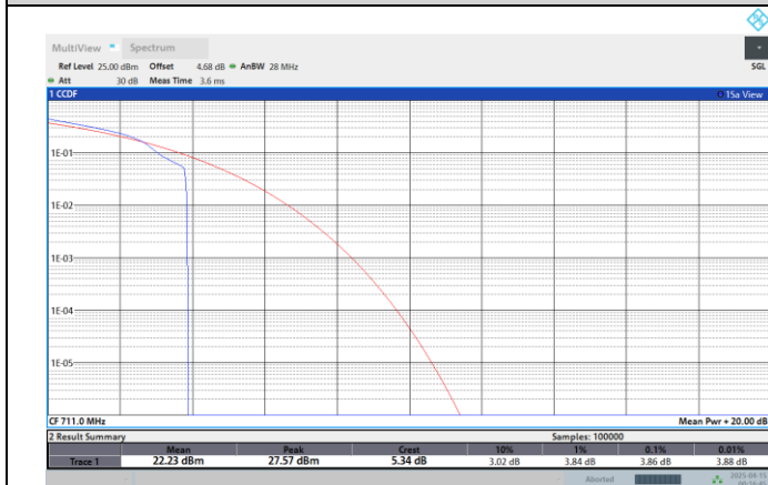
Band12-10MHz-16QAM-23130-1RB#0
