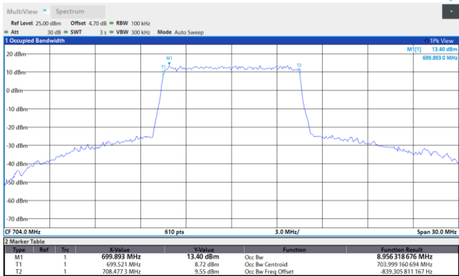
Band12-10MHz-QPSK-23095-50RB#0
