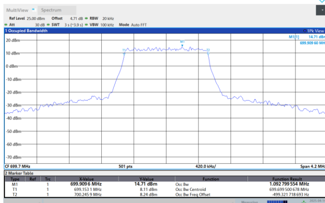
Band12-1.4MHz-16QAM-23173-6RB#0
