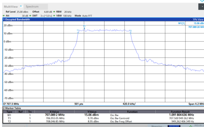
Band12-1.4MHz-16QAM-23017-6RB#0
