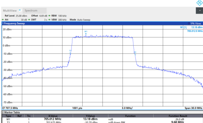
Band12-10MHz-16QAM-23095-50RB#0
