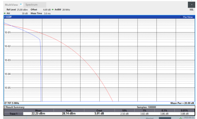
Band12-10MHz-QPSK-23130-50RB#0
