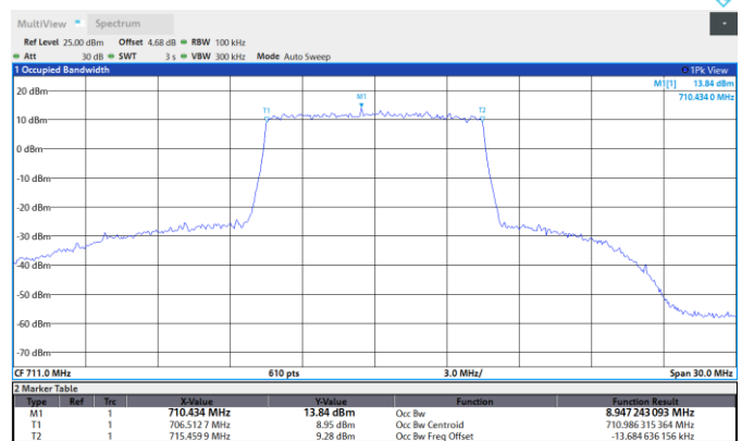
Band12-10MHz-16QAM-23130-50RB#0
