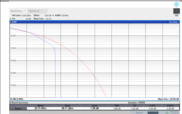
Band71-20MHz-16QAM-133372-100RB#0
