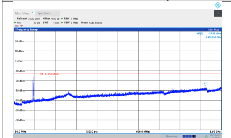
Band71-15MHz-QPSK-133397-1RB#0-Range:30~6990MHz
