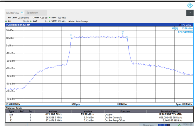
Band71-10MHz-16QAM-133422-50RB#0
