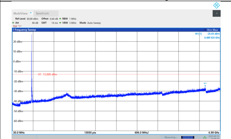
Band71-20MHz-QPSK-133222-1RB#0-Range:30~6990MHz
