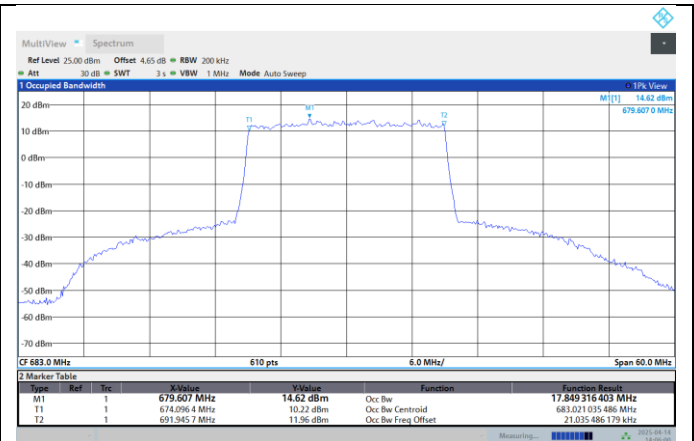
Band71-20MHz-16QAM-133222-100RB#0
