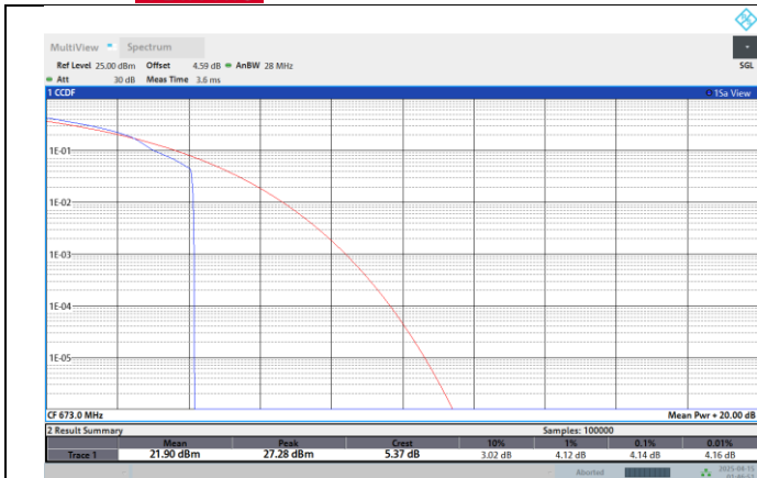
Band71-20MHz-16QAM-133297-1RB#0
