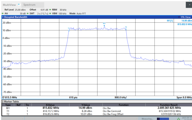
Band26-3MHz-QPSK-26775-15RB#0
