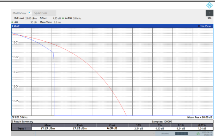
Band26-5MHz-16QAM-26715-25RB#0
