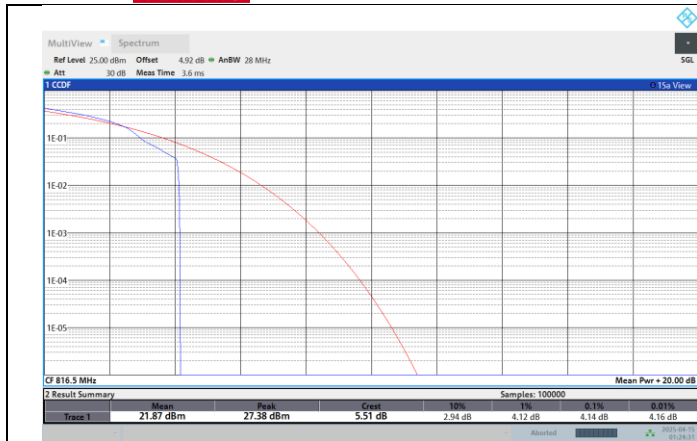
Band26-5MHz-16QAM-26740-1RB#0
