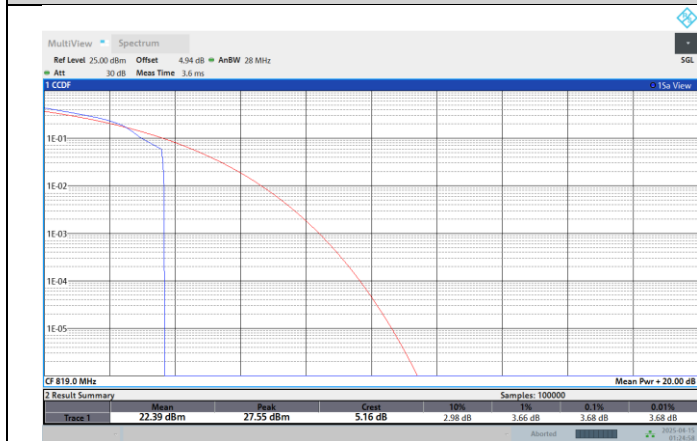
Band26-5MHz-16QAM-26765-1RB#0
