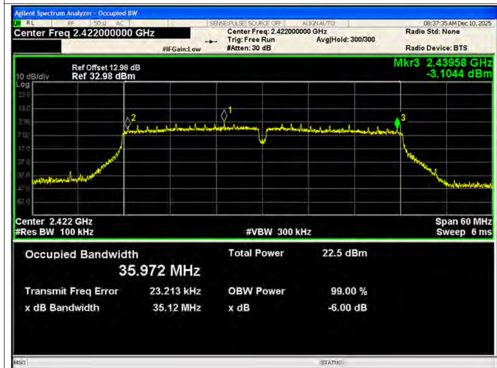
-6dB Bandwidth NVNT n40 2422MHz Ant1
