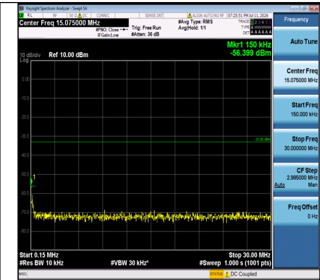
Band IV-1312-0.15~30MHz-PASS
