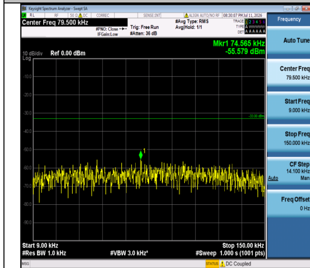
Band V-4182-0.009~0.15MHz-PASS
