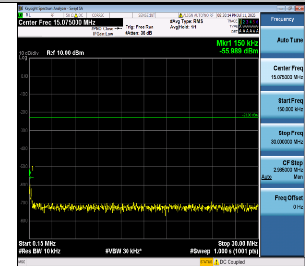
Band V-4182-0.15~30MHz-PASS
