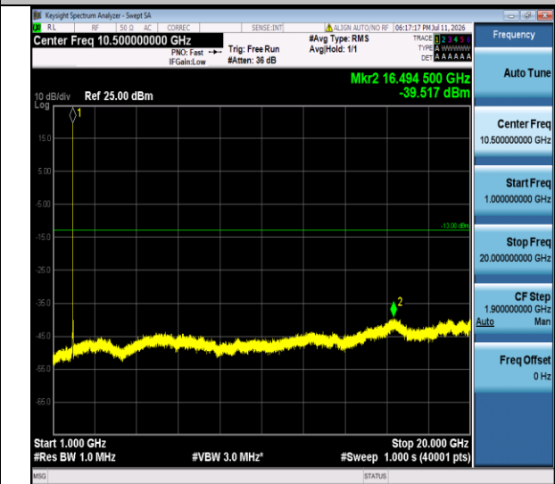
Band II-9538-1000~20000MHz-PASS
