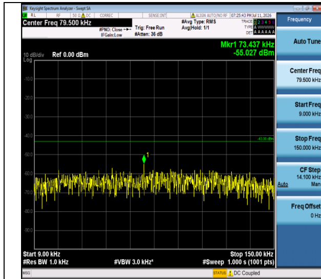
Band IV-1312-0.009~0.15MHz-PASS
