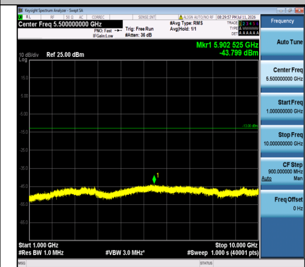
Band V-4132-1000~10000MHz-PASS
