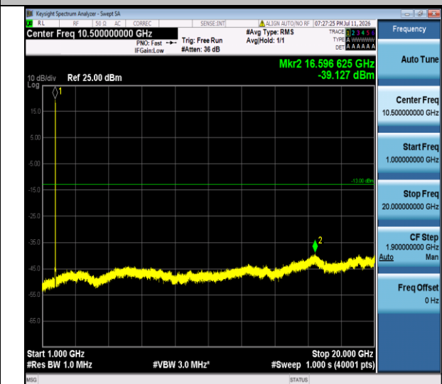
Band IV-1513-1000~20000MHz-PASS
