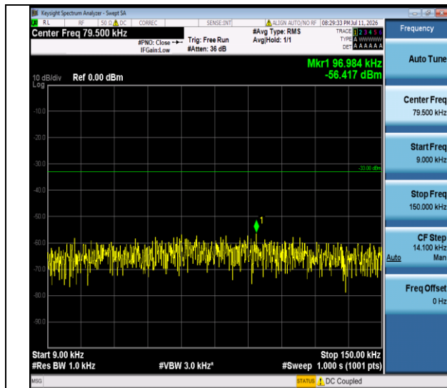
Band V-4132-0.009~0.15MHz-PASS
