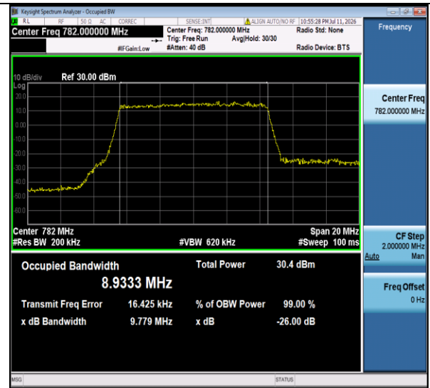
Band13-10MHz-16QAM-23230-50RB#0-PASS
