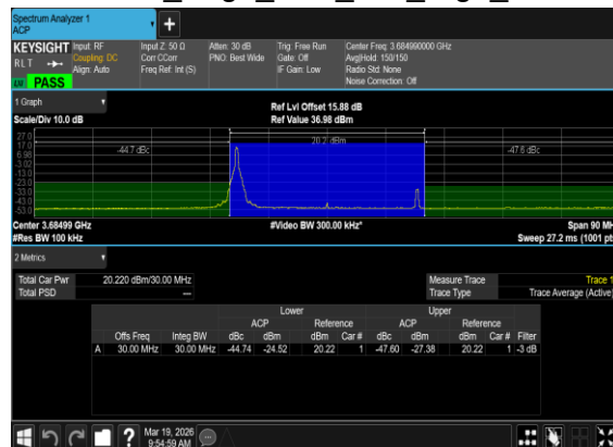
N48(30M)_DFT-s-OFDM_PI_2- BPSK_Edge_1RB_Left_High_CH
