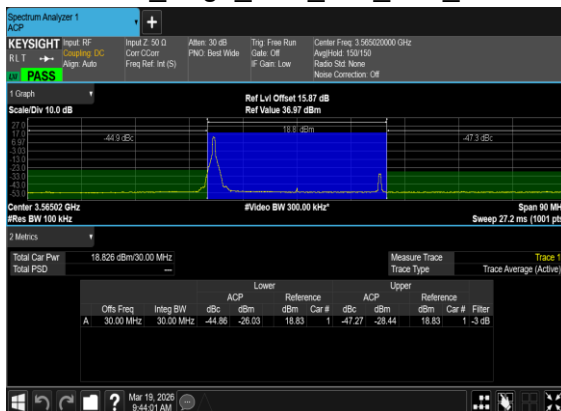
N48(30M)_DFT-s-OFDM_PI_2-BPSK_Edge_1RB_Left_Low_CH
