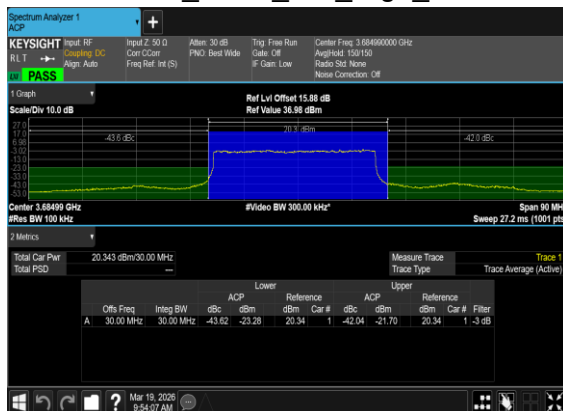
N48(30M)_DFT-s-OFDM_PI_2- BPSK_Outer_Full_High_CH
