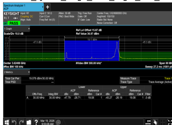
N48(30M)_DFT-s- OFDM_QPSK_Edge_1RB_Right_Mid_CH
