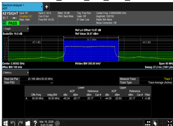
N48(30M)_DFT-s-OFDM_PI_2-BPSK_Outer_Full_Low_CH
