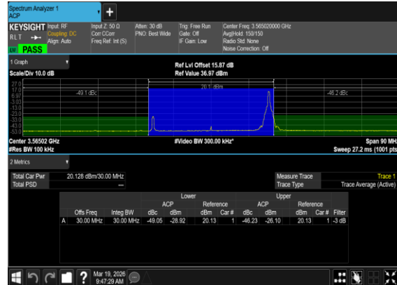
N48(30M)_DFT-s- OFDM_QPSK_Edge_1RB_Right_Low_CH
