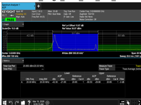
N48(20M)_DFT-s-OFDM_PI_2-BPSK_Edge_1RB_Left_Mid_CH
