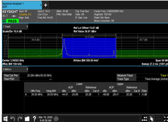
N48(30M)_DFT-s- OFDM_QPSK_Edge_1RB_Left_Low_CH
