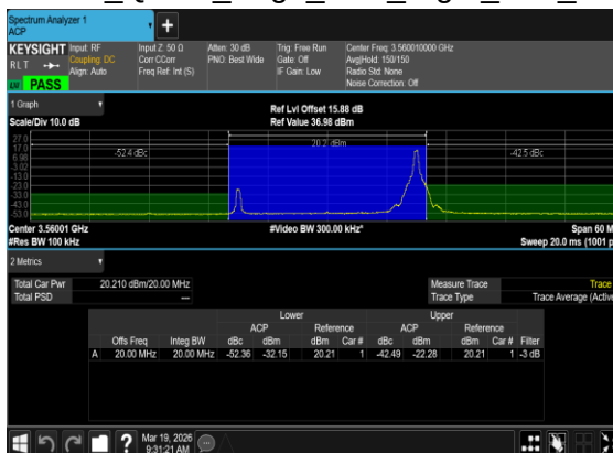
N48(20M)_DFT-s-OFDM_QPSK_Edge_1RB_Right_Low_CH
